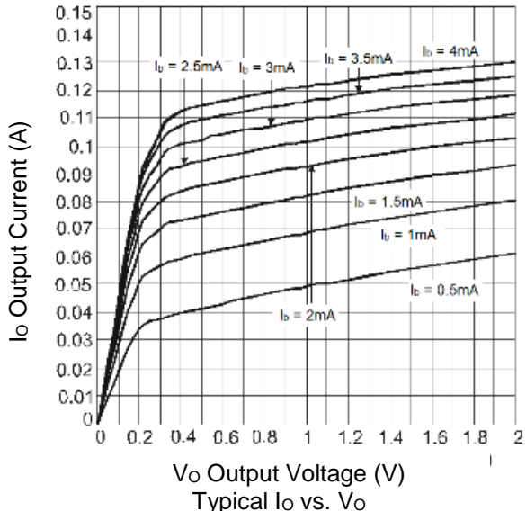
Typical I_o vs. V_o
