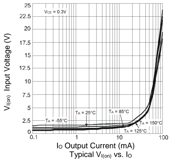
Typical V_i vs. I_o
